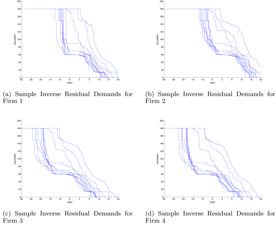
Figure 3. : Inverse Residual Demand Data
